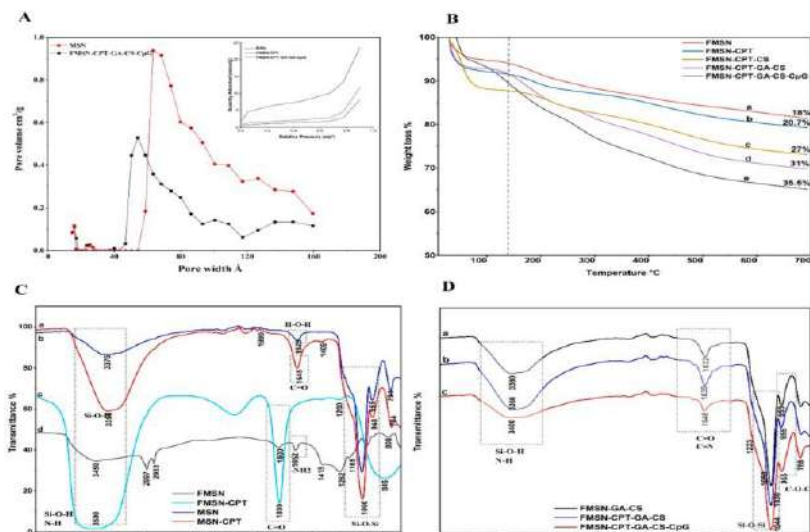
Fig. 3: (A) Brunauer-Emmett-Teller (BET) surface characterization (B) Thermogravimetric Analysis TGA thermal behavior of NPs (C, D) Fourier-Transform Infrared Spectroscopy (FTIR), Chemical characterization.
