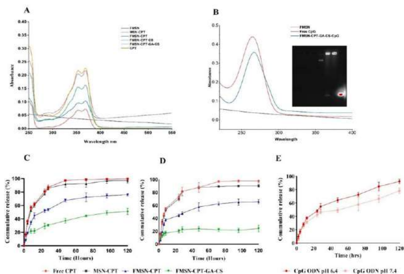
Fig. 4: (A) UV spectrum of CPT, blank FMSN, MSN-CPT, FMSN-CPT, FMSN-CPT-CS, FMSN-CPT-GA-CS (B) UV spectrum of CpG ODN and gel electrophoresis detection of CpG ODN (C, D) Cumulative release of CPT, MSN-CPT, FMSN-CPT and FMSN-CPT-GA-CS at pH 6.4 and pH 7.4, respectively, (E) Cumulative CpG ODN release at pH 6.4 and pH 7.4.
