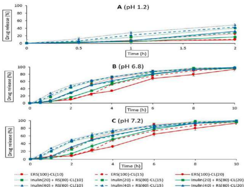
Fig. 1: The drug release profile from the pellets coated under the experimental design conditions at various pH conditions. CL: coating level.
